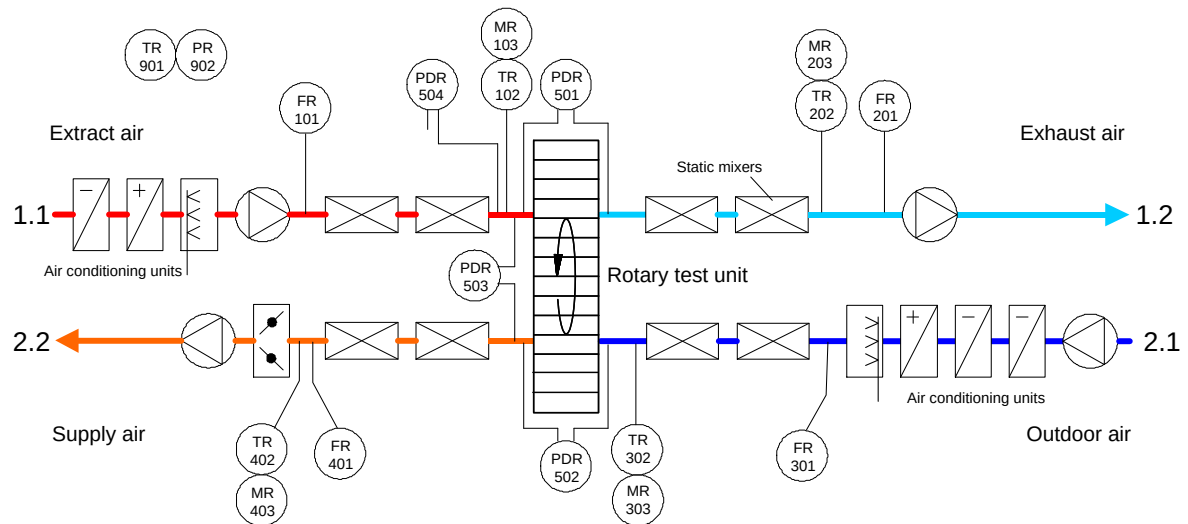
Figure 13: Heat recovery test rig
